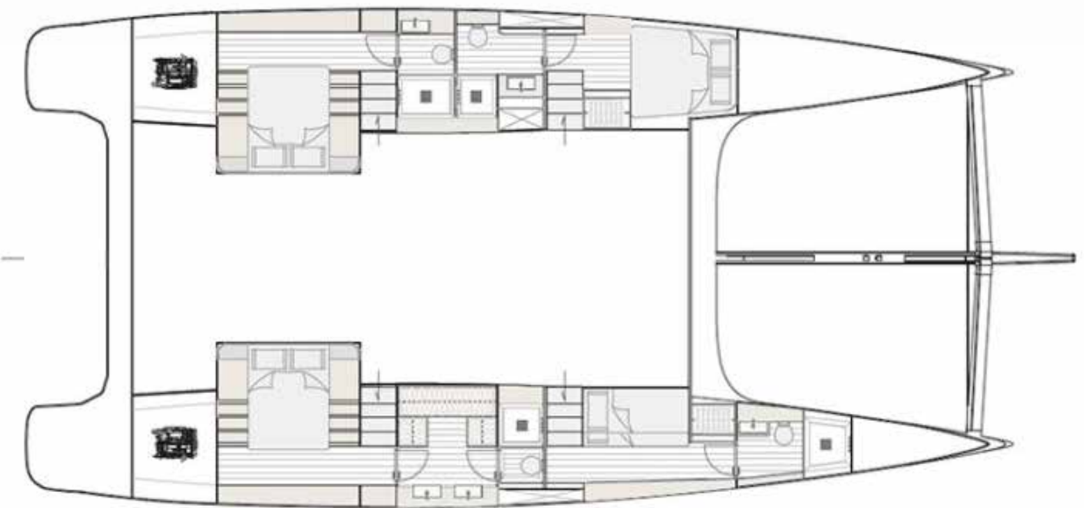
MAIN DECK GA.
